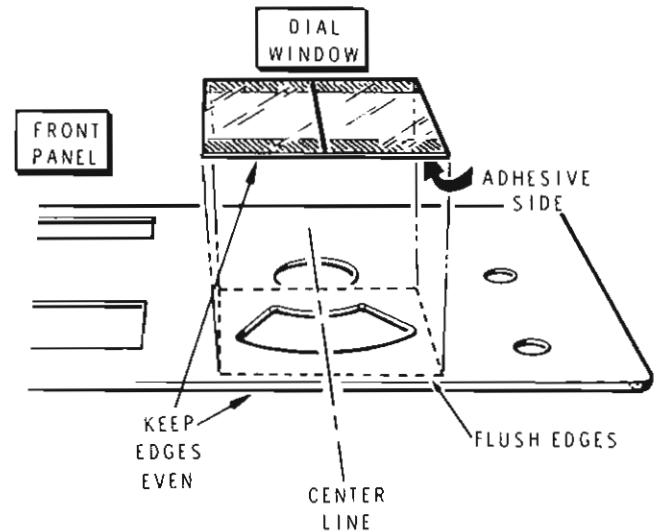
Detail 4-5A
