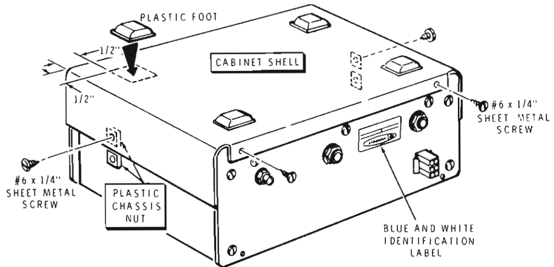
PICTORIAL 5-3
