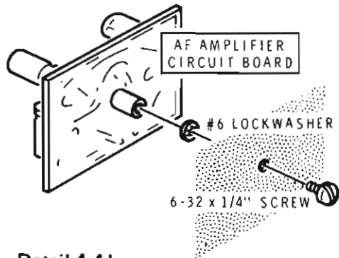
Detail 4-4J
