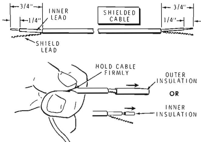
Detail 3-2A
