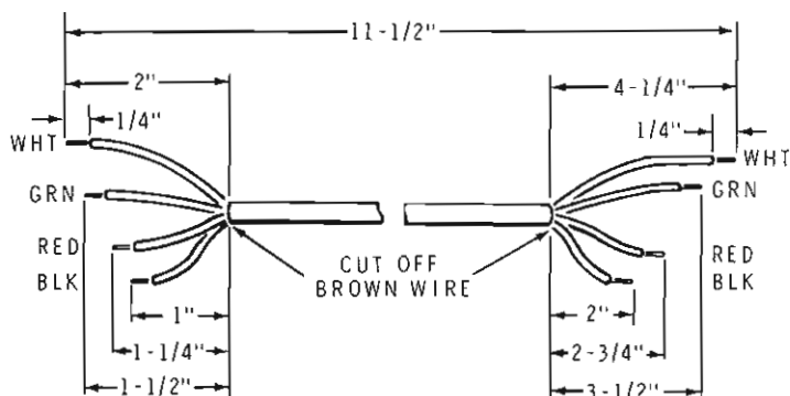
Detail 3-1B
