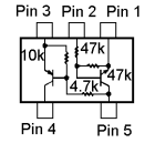
FMC5A (C5) (Q5003, 5004)
