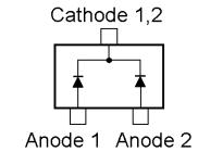
DAN202U (N) (D5011, 5018)
