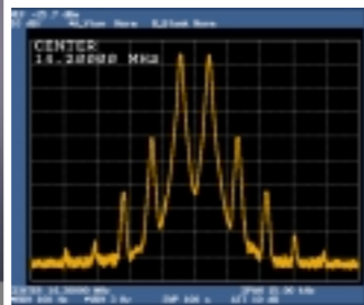
Typical TX IMD: Class A (25W Output)
