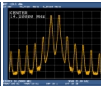
Typical TX IMD: Class AB (100 W Output)
