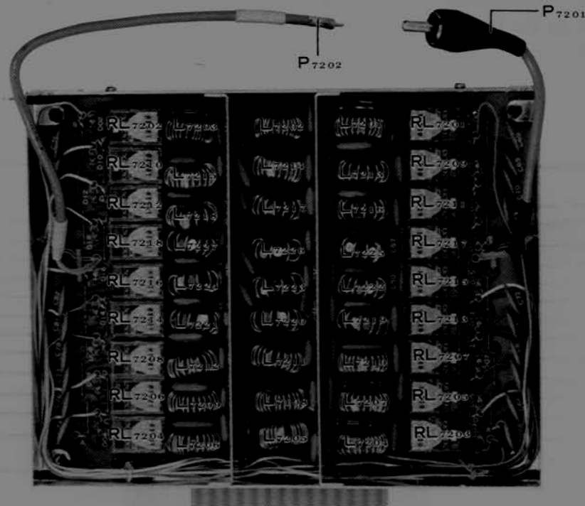
LPF UNIT (PB-2259)
