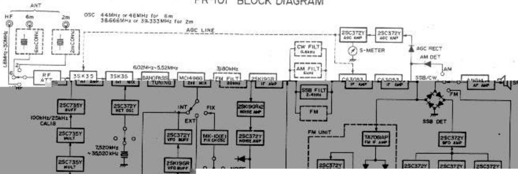
FR-101 BLOCK DIAGRAM
