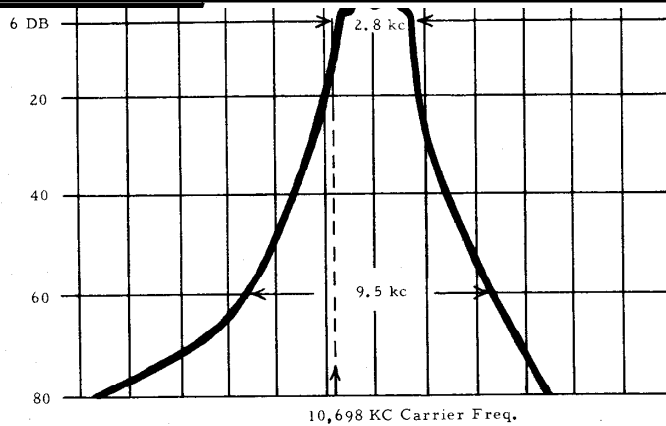
FIGURE 3 CRYSTAL FILTER, TYPICAL CHARACTERISTIC
