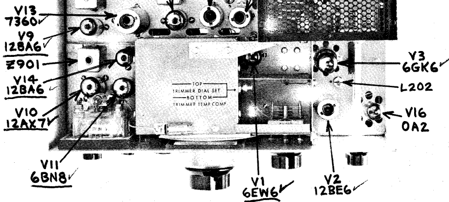
FIGURE 4 TOP VIEW MODEL 250 TRANSCEIVER
