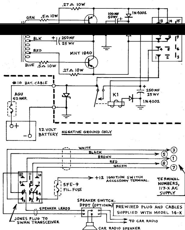
SWAN MODEL 14-X D.C. MODULE
