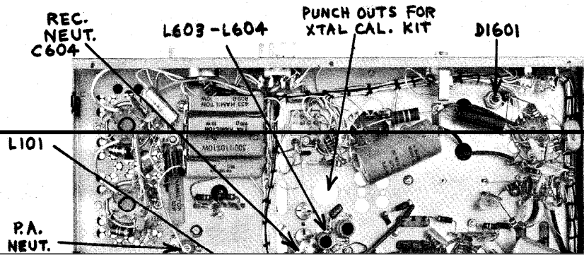
FIGURE 5 BOTTOM VIEW MODEL 250
