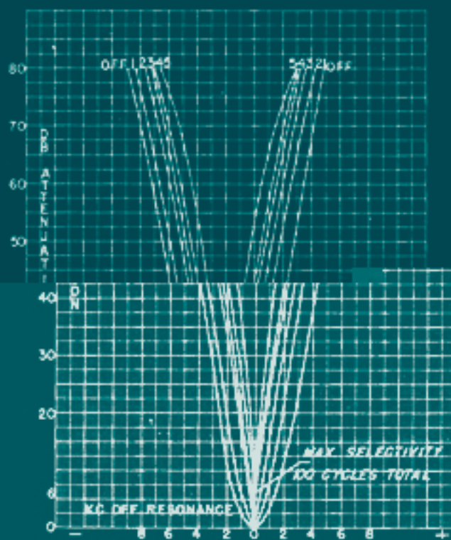
Figure No. 1. Crystal Filter Selectivity Curves
