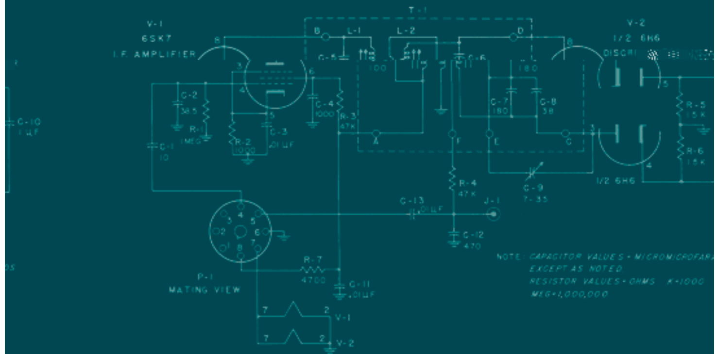
Figure No. 16. Schematic Diagram, NFM-83-50 Adaptor
