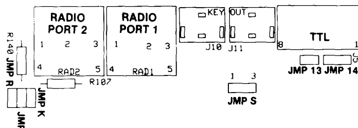
FIG. 3-3 HT Special Keying Circuit
