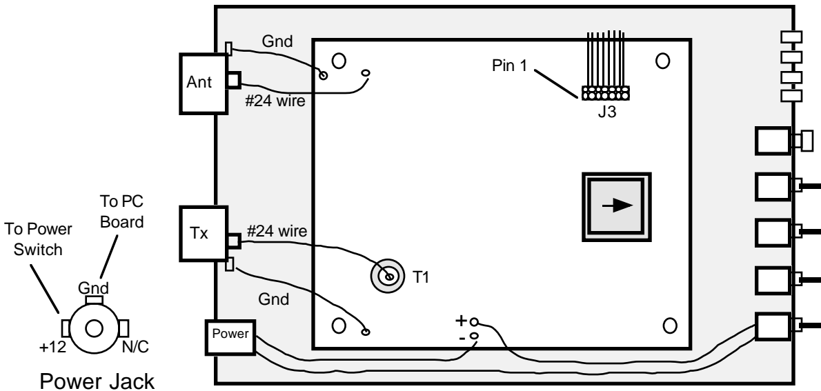
Fig. 10 Chassis Top View
