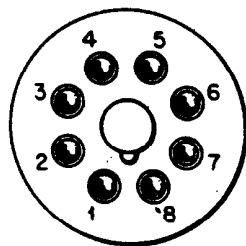
OCTAL BASE
