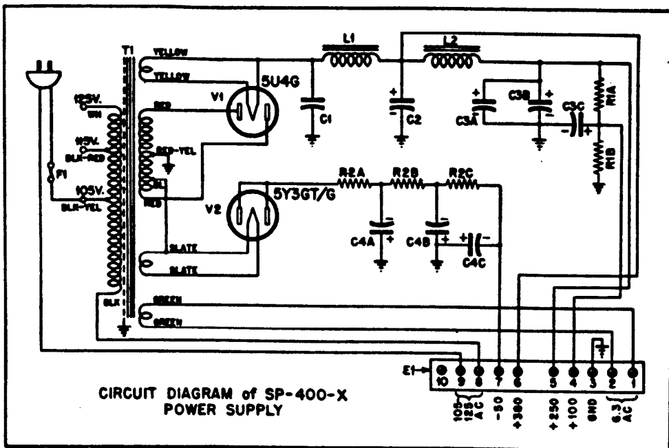
FIG. 10— Power supply diagram.
