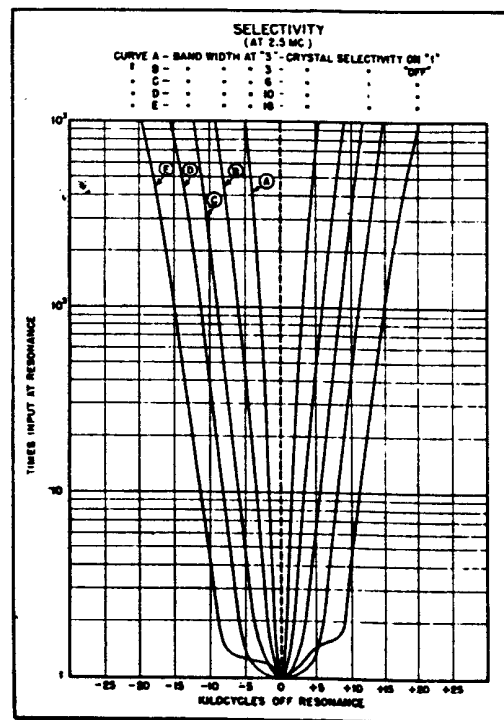
FIG. 8—Selectivity curves.
