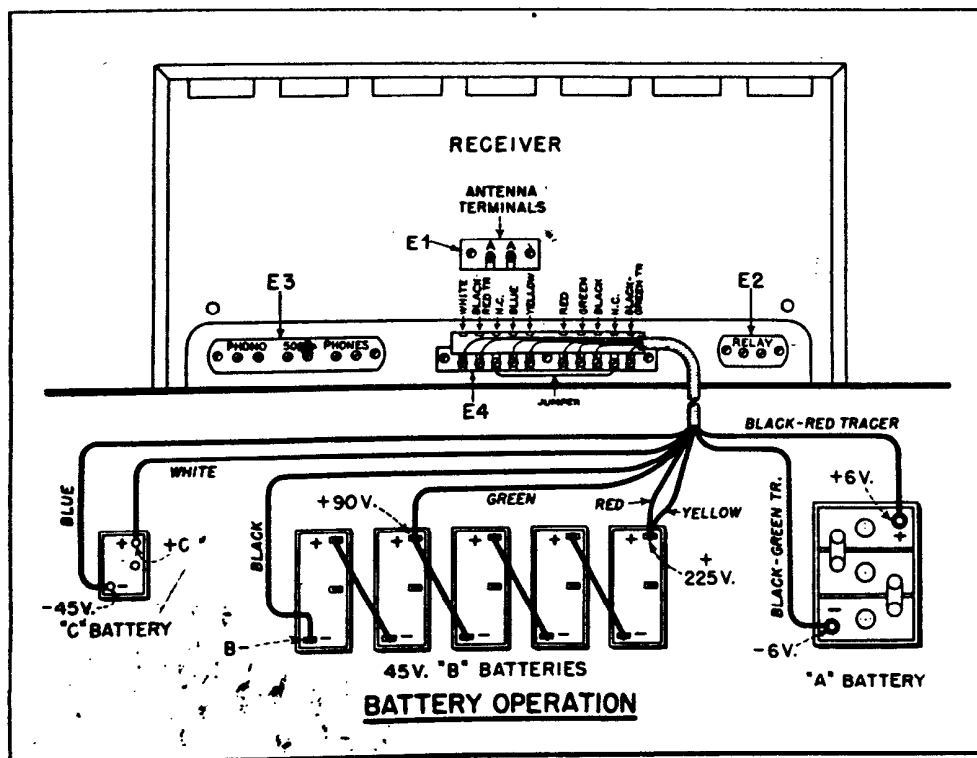
FIG. 4—Connections for power cable—battery operation.
