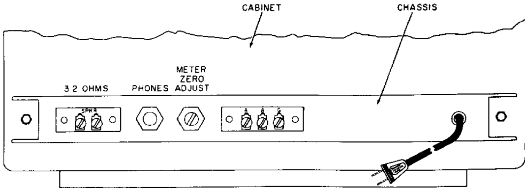
FIGURE I-1. REAR CONNECTIONS.
