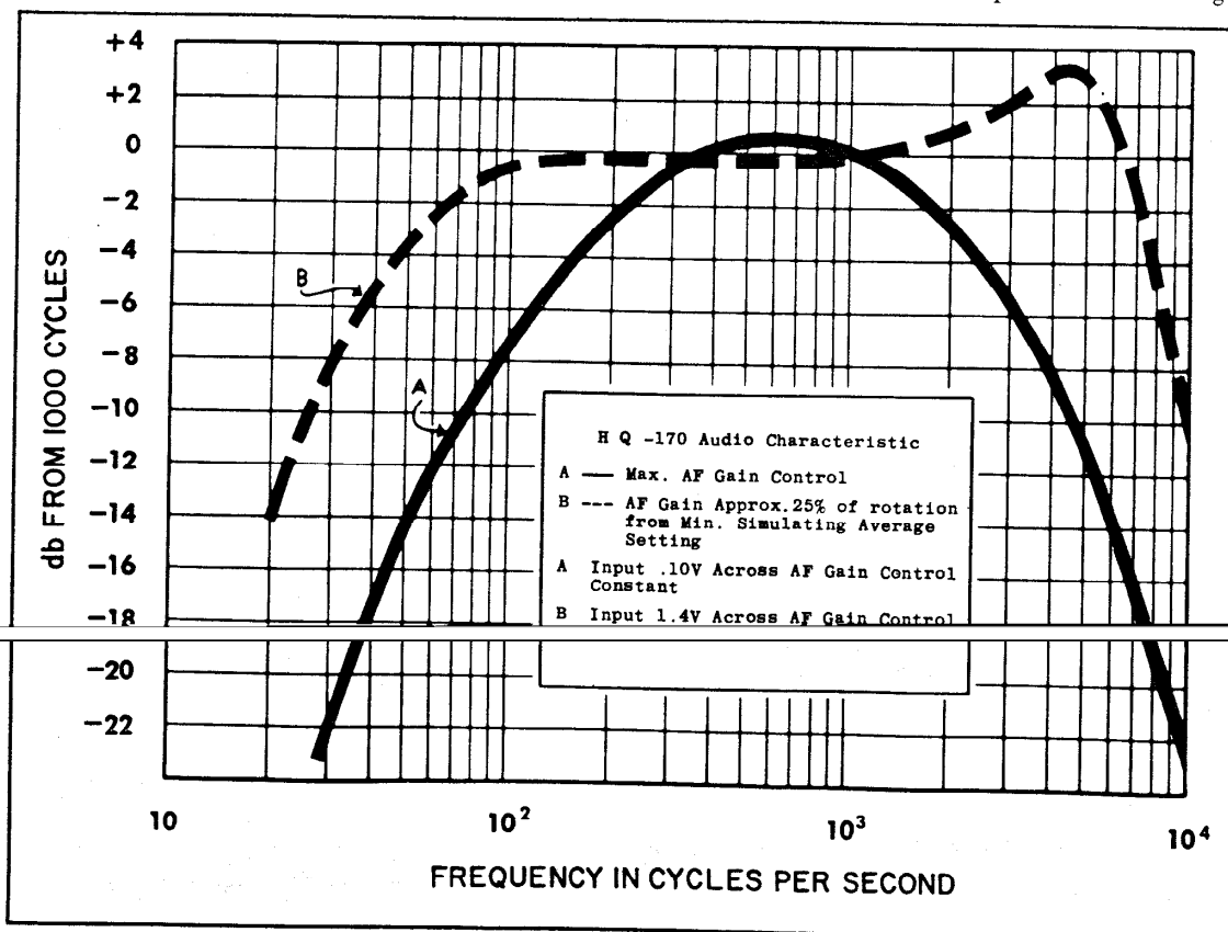
Figure 8. Auto-Response Curve
