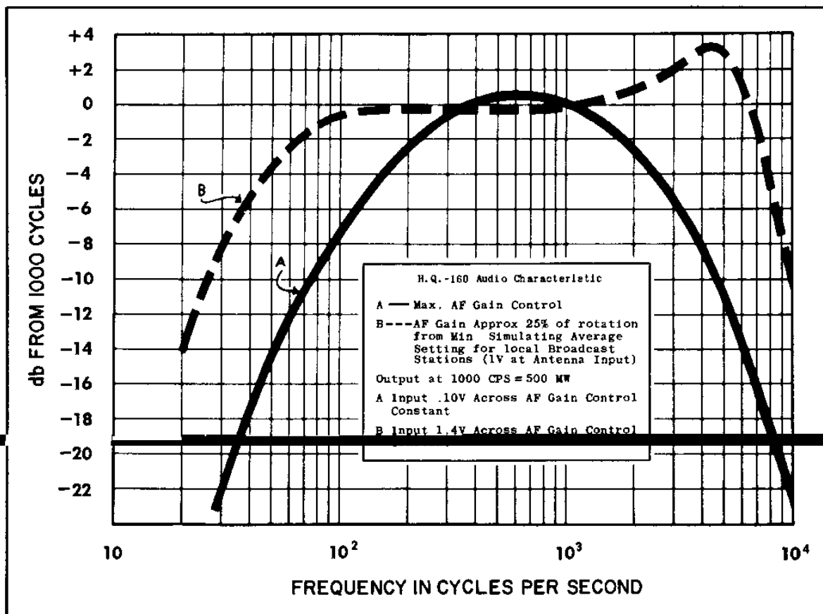
Figure 6. Auto-Response Curve
