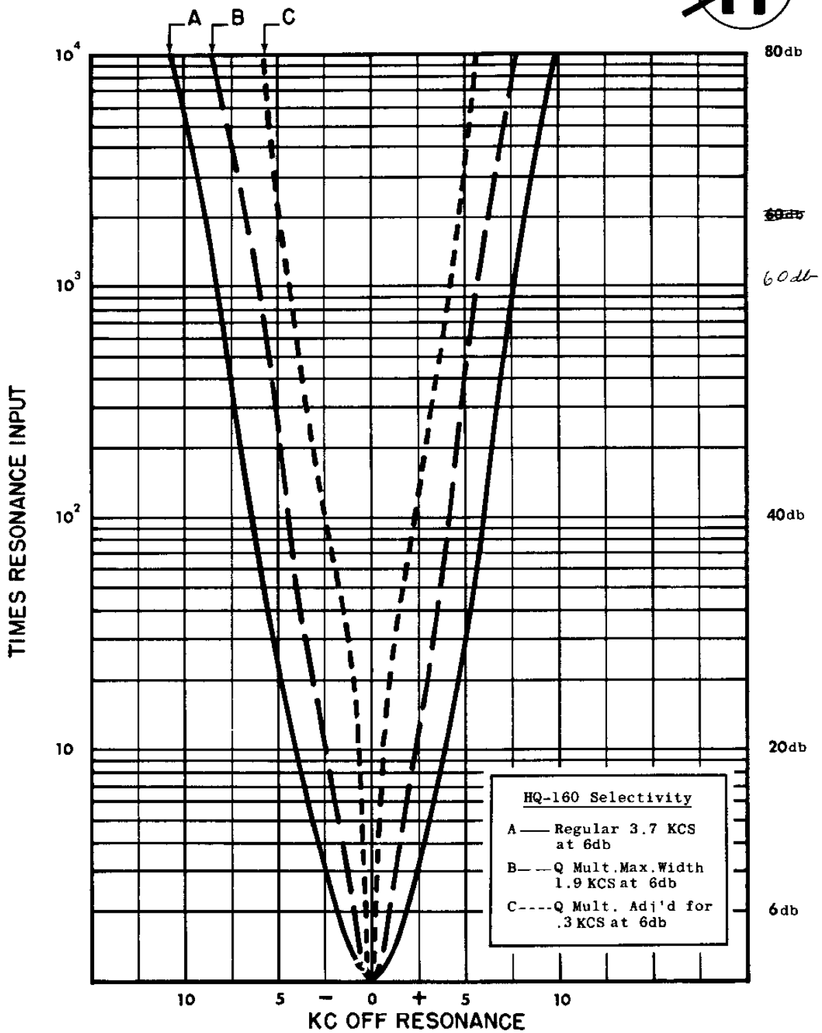
Figure 11. Selectivity Curves
