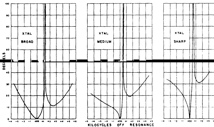
FIG. 4—CRYSTAL SELECTIVITY
