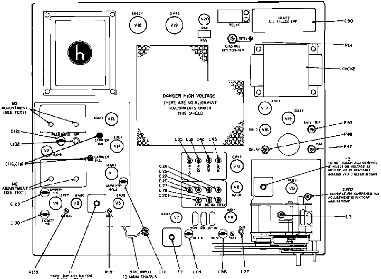
Figure 8. Top Chassis Alignment Points
