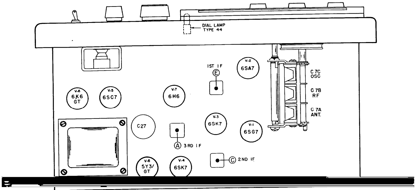
Fig. 4. Top View of Chassis Showing Location of Alignment Adjustments, Tubes and Dial Lamp
