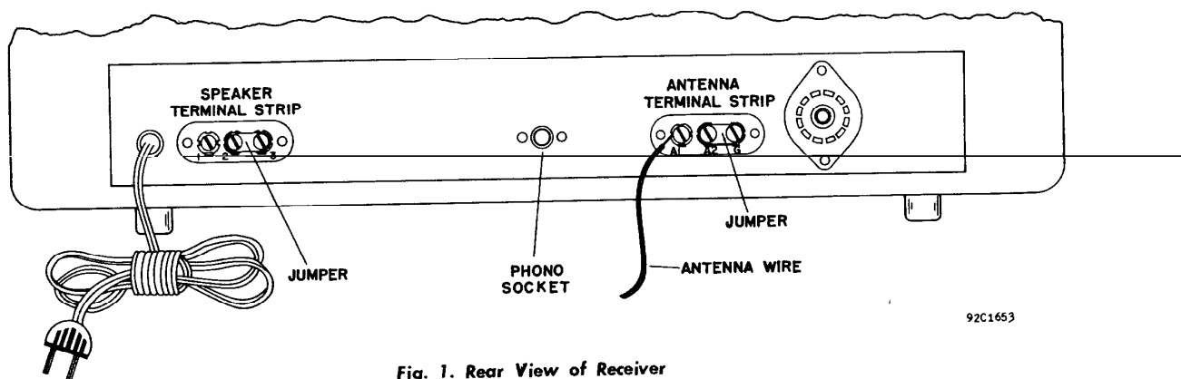
Fig. 1. Rear View of Receiver
