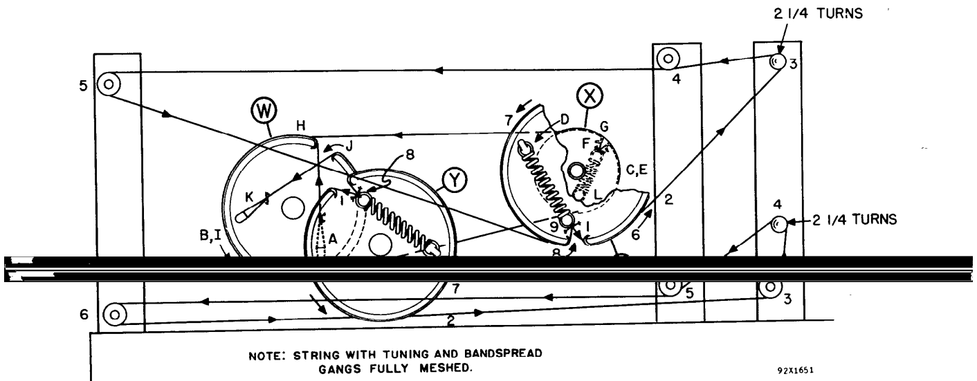
Fig. 2. Dial Cord Stringing Diagram
