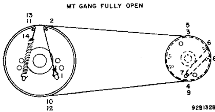
FIG. 5. MAIN TUNING GANG DRIVE STRINGING PROCEDURE
